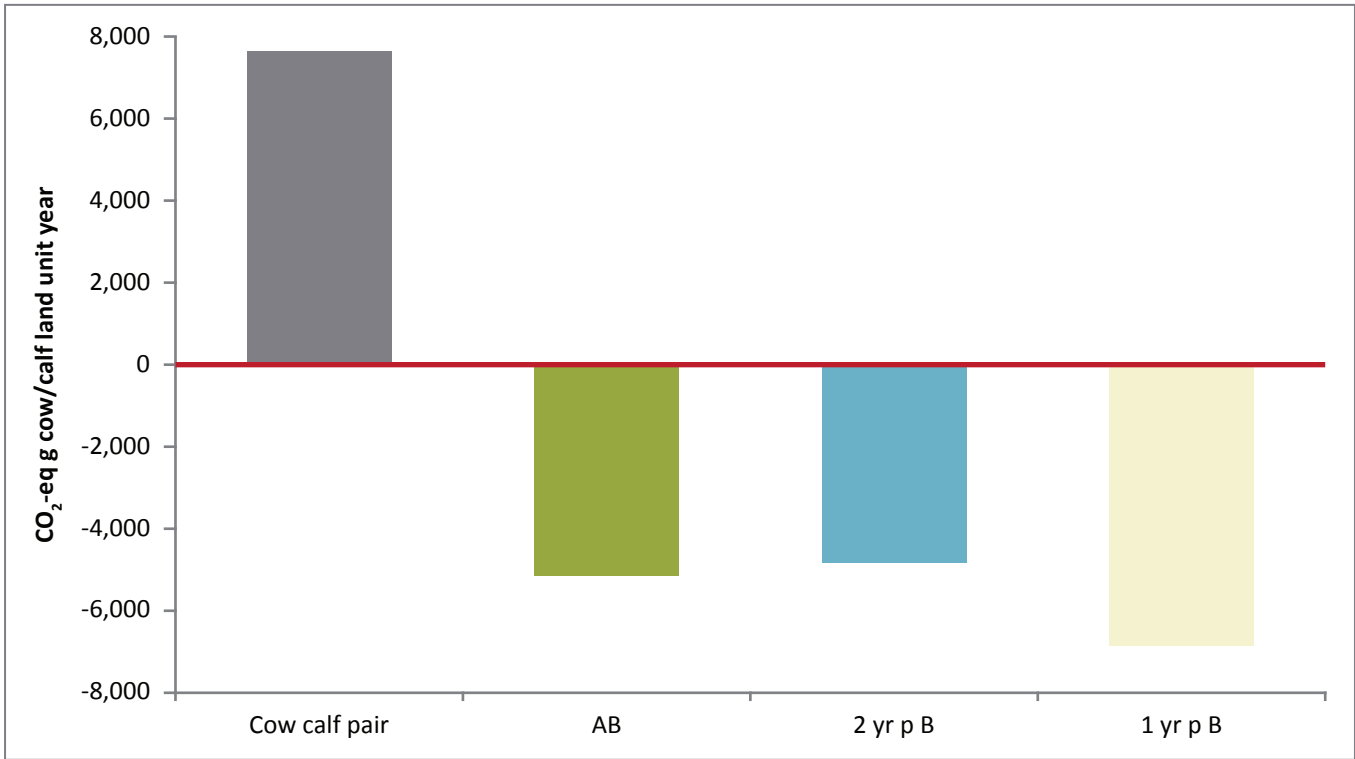
Figure 2. Managed grassland soil capacity to capture \text{CH}_4 and \text{N}_2\text{O} emissions from three watersheds under annual burning (AB) and patch burning on a 3-year basis: 2-years post-burning (2 yr p B) and 1-year post-burning (1 yr p B). The cow-calf pair bar indicates emission from the animal during the grazing season. Sources: Rivera-Zayas et al., 2016; Todd et al., 2016.
